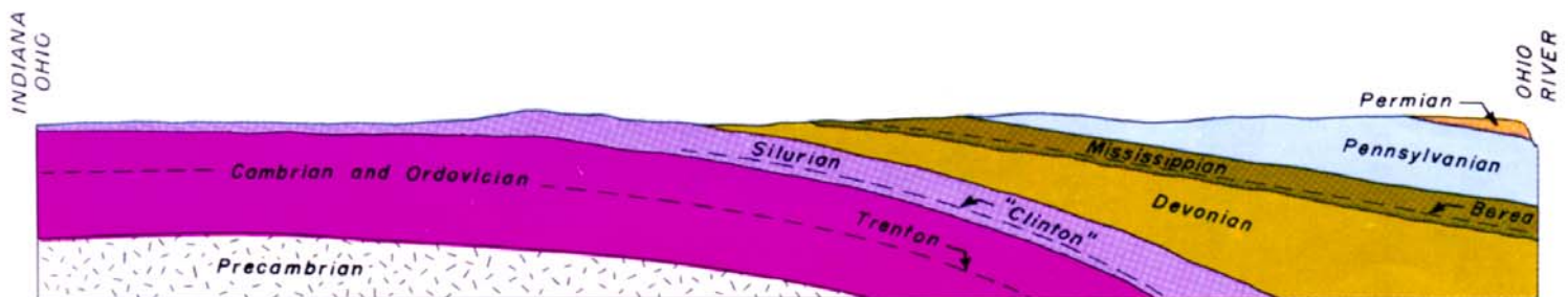
GEOLOGIC MAP AND CROSS SECTION OF OHIO
